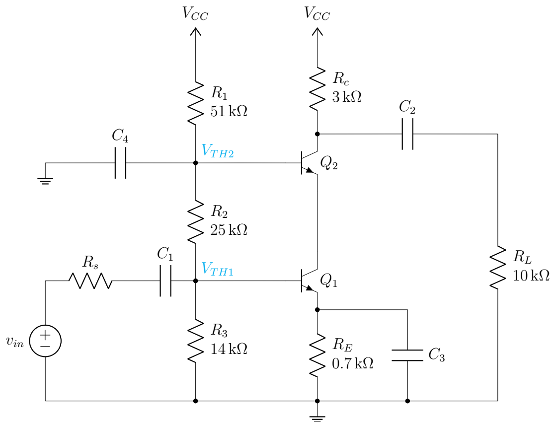
Figure 1: Amplificador cascode
